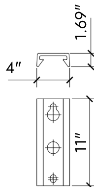
Mounting Plate Detail
