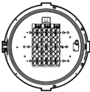
Bottom View w/ Globe Removed
