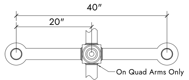
Top View of Arm
