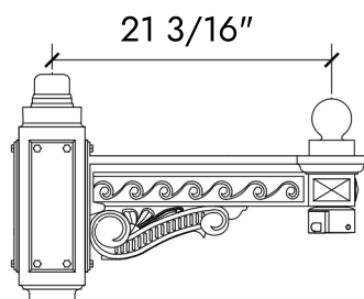
Journal Square Tri Bracket
