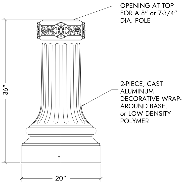
Montclair Wrap Around Base Available in Cast Iron, Aluminum or Linear Low Density Polyethylene
