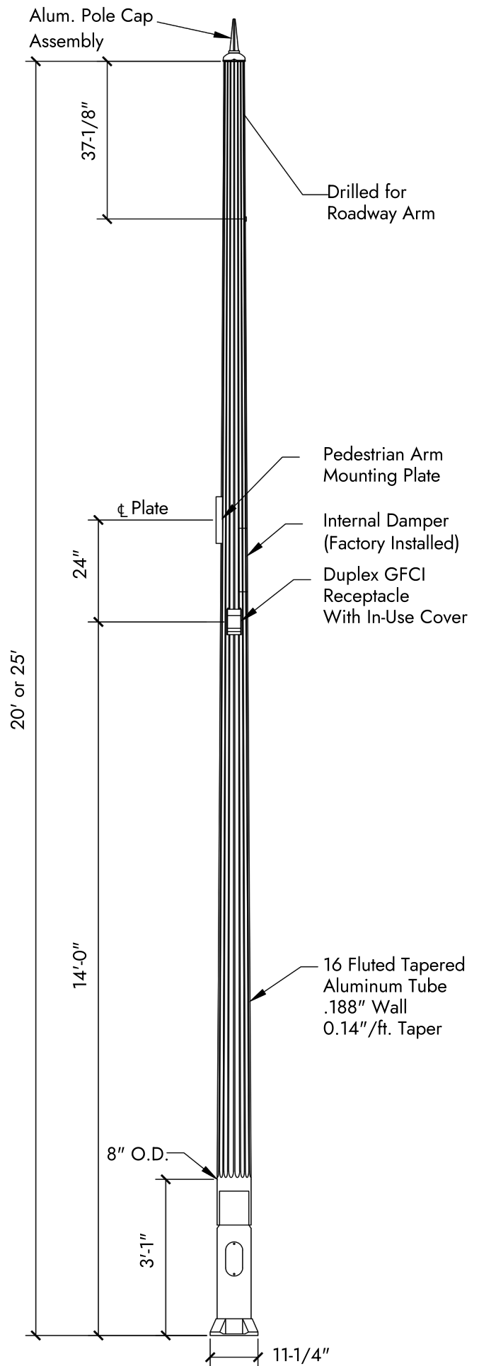
Tall Deco Fluted Pole w. Ped Plate Available with and without Ped, Smooth or Fluted Shaft
