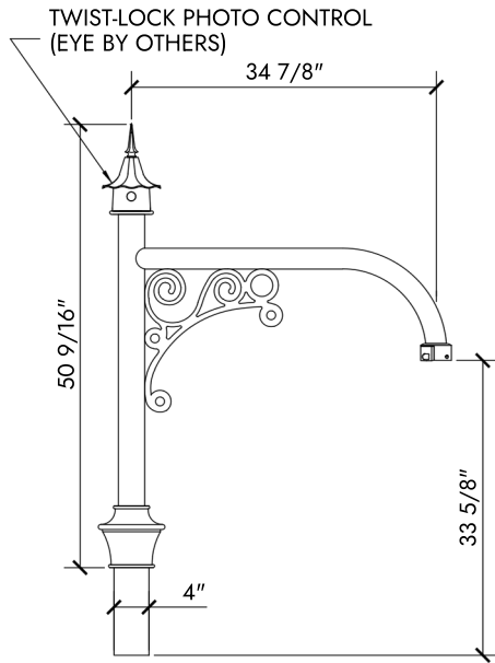
Camden Arm Bracket
