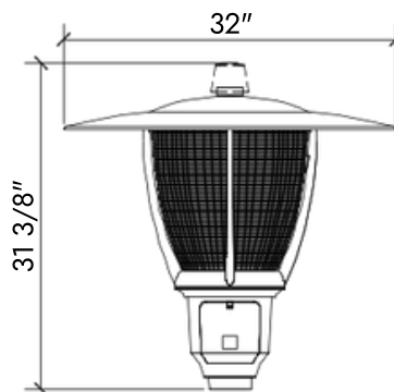
Contempo II LED
