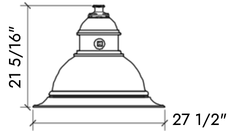
Domus LED Available in Black or Green in Type 4 or 5
