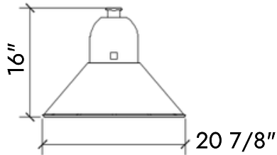
Small Tear Drop Available in Black or Federal Highway Green With or Without Brim in Type 3 or 5
