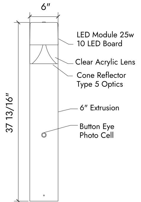
Commercial Bollard in Black
