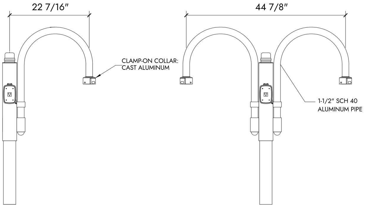
Hudson Short Arm
