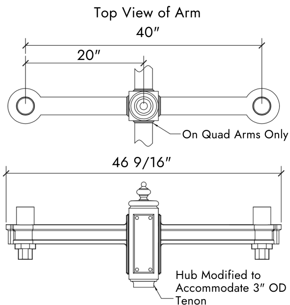
Regency 2 Twin Arm
