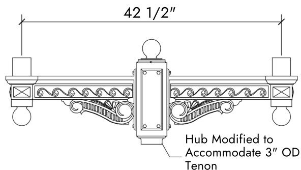
Colgate Post Top Twin Bracket
