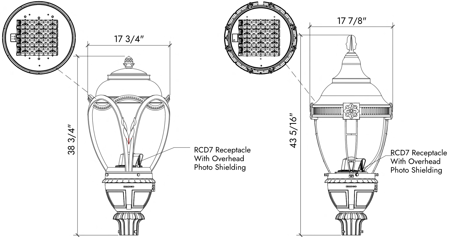
Hagerstown Full Cut-off LED
