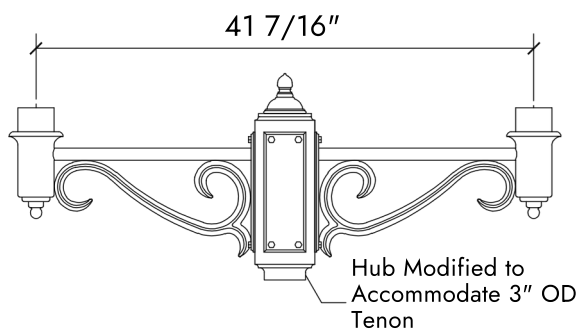
Colonial Twin Arm 39 1/4"
