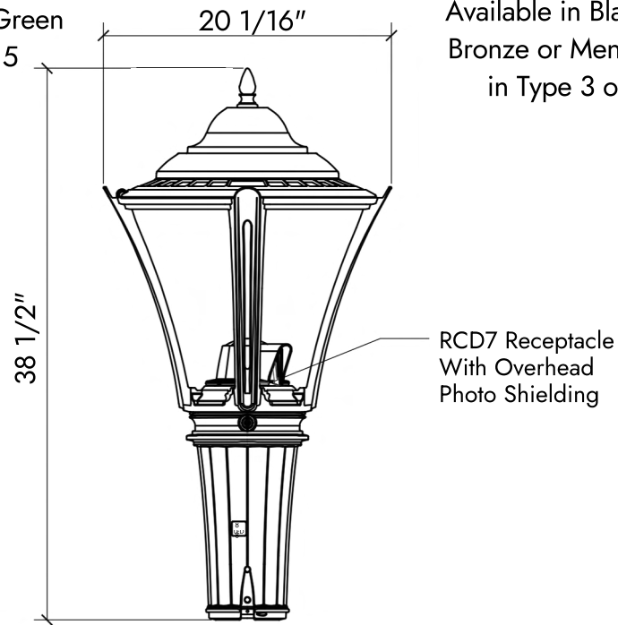
Hagerstown Full Cut-off LED
