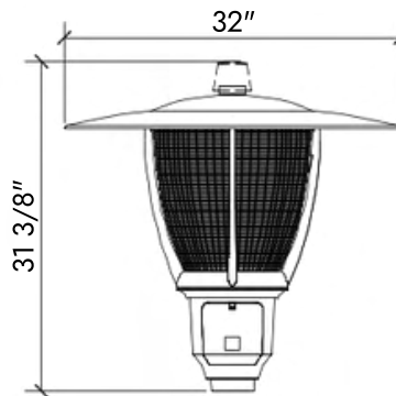
Contempo II LED Available in Black in Type 3 or 5
