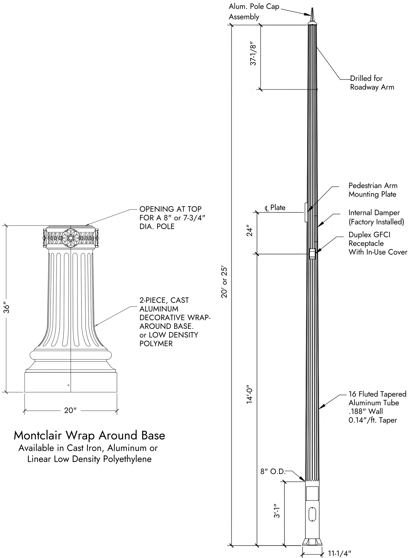
Tall Deco Fluted Pole w. Ped Plate Available with and without Ped, Smooth or Fluted Shaft
