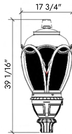
Capitol LED Available in Black or Green in Type 3 or 5
