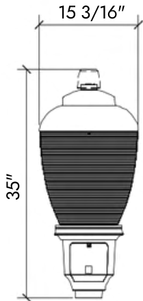
Deluxe Acorn II LED Available in Type 3 or 5
