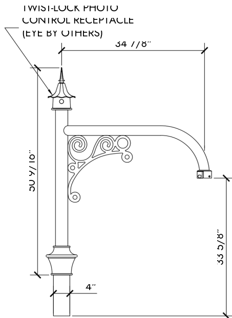
Camden Arm Bracket
