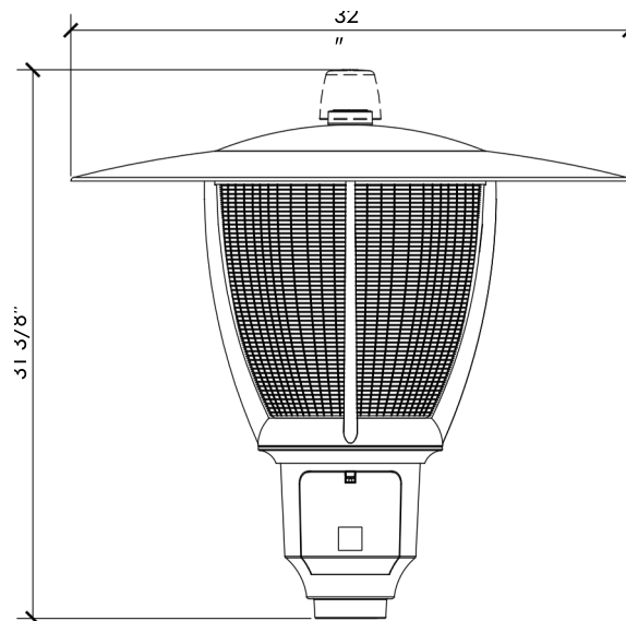
Contempo II - LED Available in Black In Type 3 or Type 5
