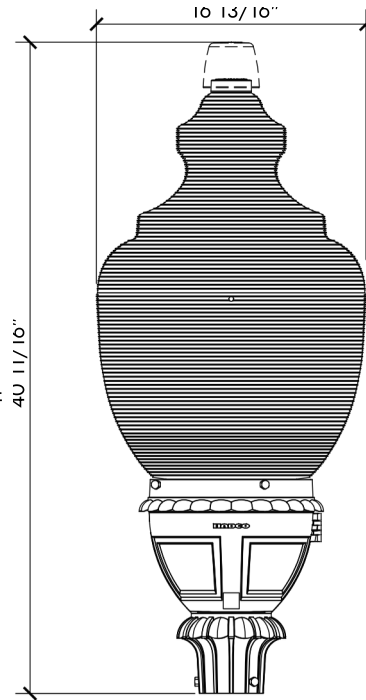
Irenton - LED
