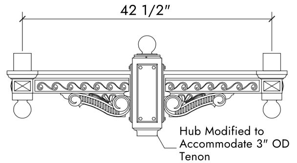
Colgate Post Top Twin Bracket
