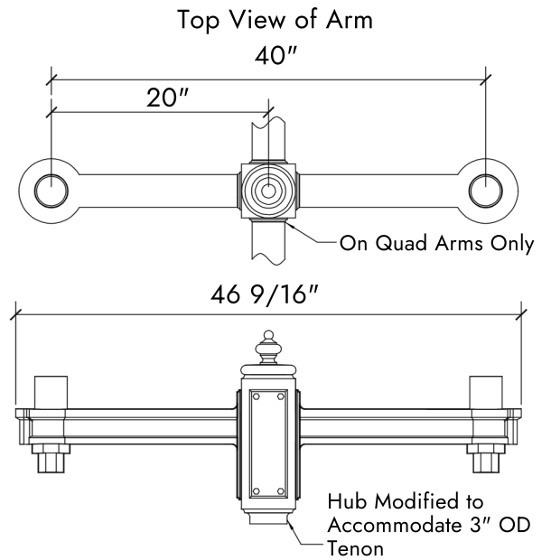
Regency 2 Twin Arm
