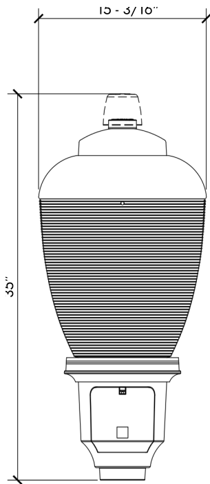
Deluxe Acorn II - LED Available in Black In Type 3 or Type 5
