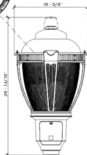
Franklin Park Cut-off - LED Available in Black in Type 5
