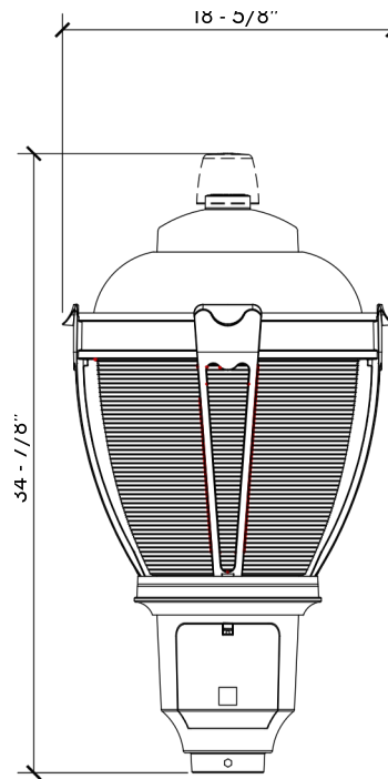
Franklin Park - LED Available in Bronze or Black, In Type 3 or Type 5
