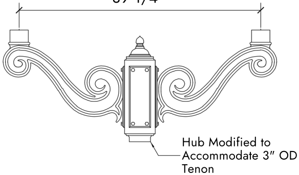
Colonial Twin Arm 39 1/4"
