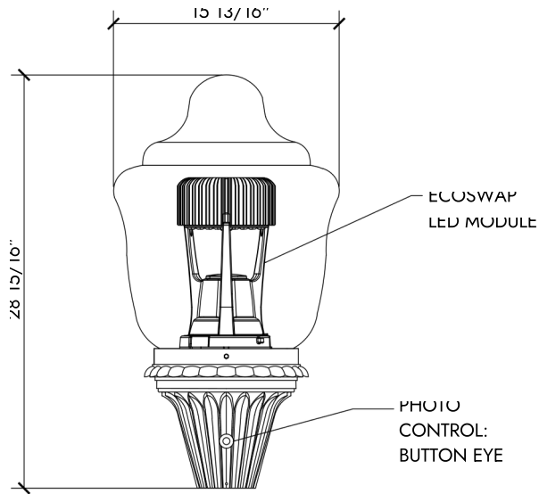
Montclair - LED
