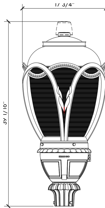
Capitol - LED Available in Black or Green In Type 3 or Type 5
