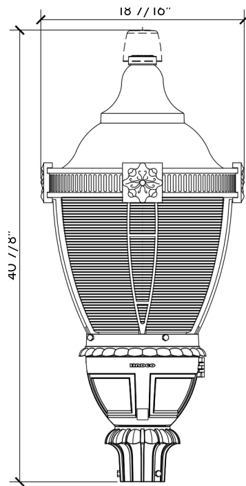
Hagerstown - LED Available in Black, Green, Bronze & Menthol Green
