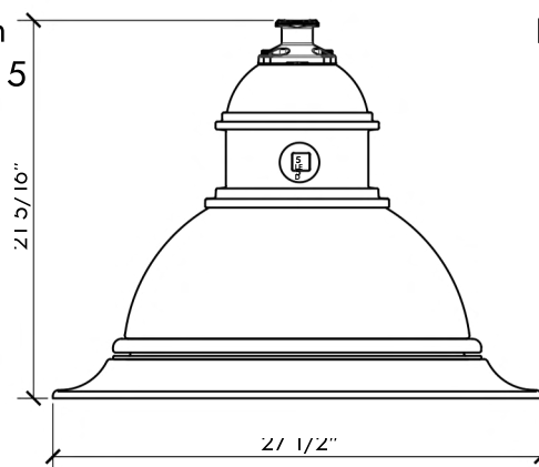
DOMUS LED Available in Black or Green In Type 4 or Type 5
