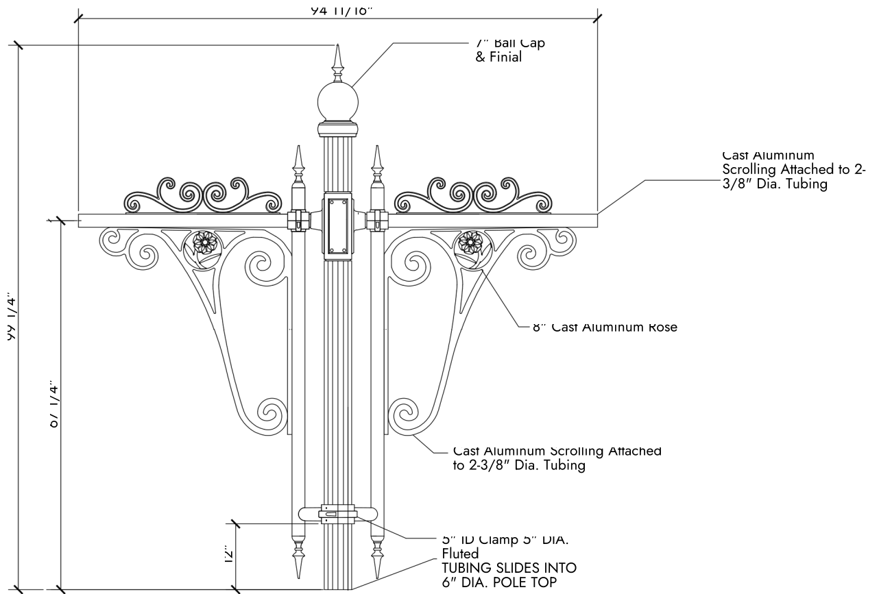
Broad Street Twin Arm
